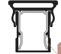
Top Rail 1.75" x 1.875" (.070")
